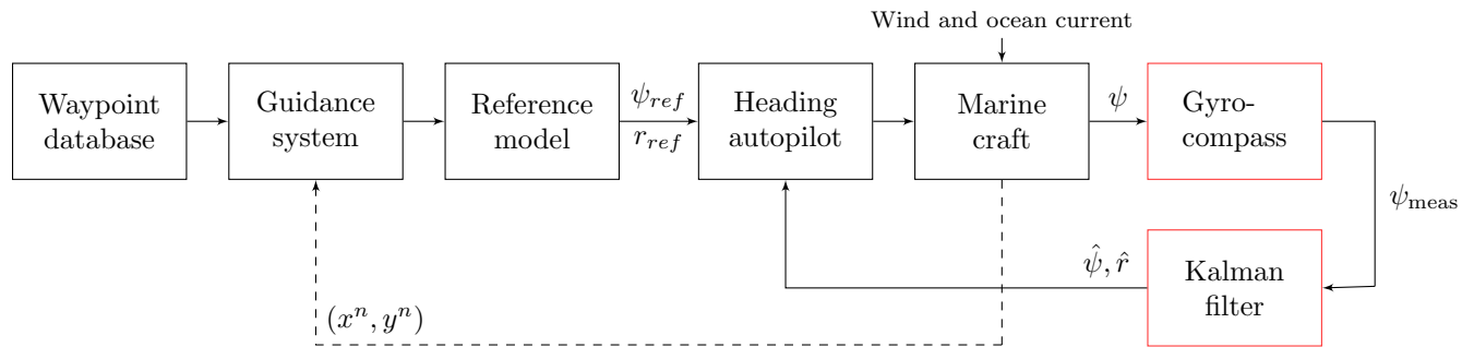
Figure 4: An overview of the guidance, navigation, and control blocks and how they interact. The navigation system (shown in red) comprises a gyrocompass and a Kalman filter and is the focus of this assignment.
