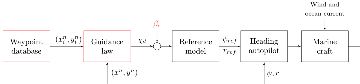
Figure 2: A block diagram illustrating the interaction between the way-points, guidance law, reference model, heading autopilot, and marine craft. The design and implementation of the way-points, guidance law and crab angle compensation (shown in red) are the main focus of this assignment.
