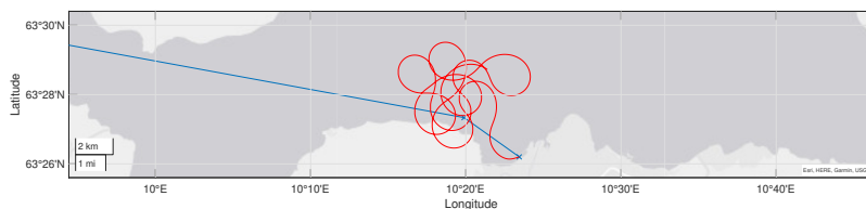
Figure 3: Unsuccessful path following due to poor tuning of the heading controller. Possible solutions: try using just PD or PID with anti-windup.
